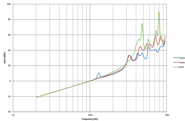
Figure 5 Normalised in-room acoustic power measurement for loudspeaker stands
