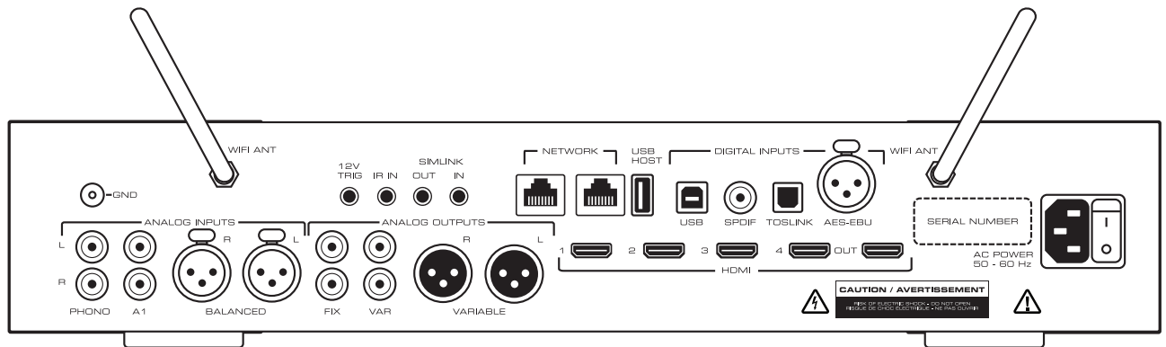
Figure 2: 390 Backpanel
