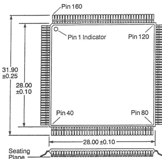
Figure 4-2. Akiko Dimensions and Pin Numbers
