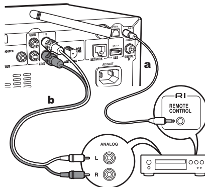
a RI Cable, b Analog Audio Cable
