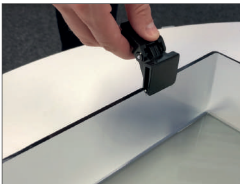
Fig. 2 Inserting the hood hinges
