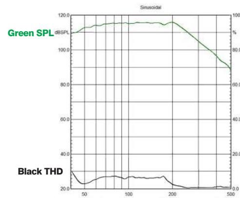
Sound Pressure Level and Distortion
