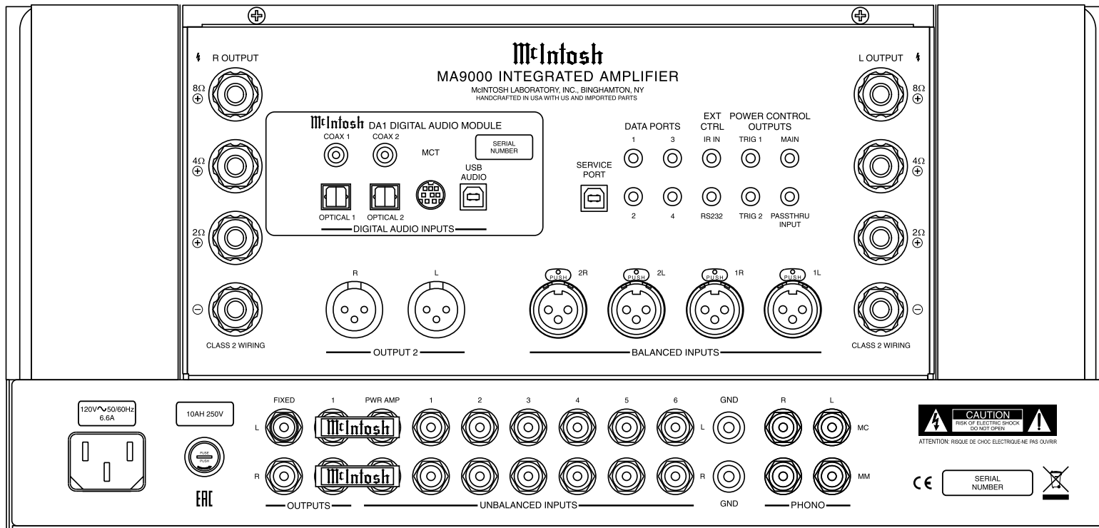
MA9000 Integrated Amplifier
